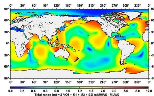
Figure 3.5: Tides over the world (Romano Lecture Notes, 2026).
