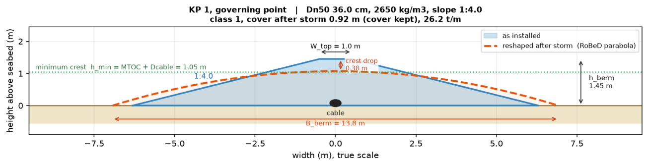
Figure 8.13: Cross-section of the normal-density design of Project C at KP 1, drawn at the rock the tool asks for rather than at the proposed grading. See the note below Table 8.11.
