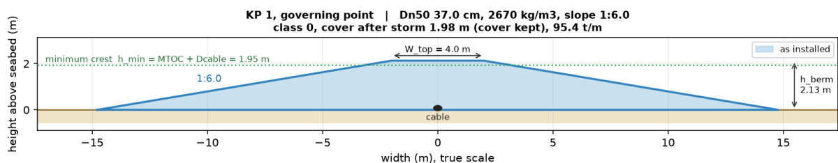
Figure 8.6: Cross-section of the berm as installed for Project B at KP 1, at the rock of the built design. The berm is class 0 under the design condition, so the as-built and the post-storm profile are the same.
