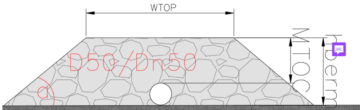
Figure 2.4: The rock berm and the terms used in this thesis, with the top width, the side slope, the berm height, the cover on the cable, the armour and the underlayer. (W.Pol)
