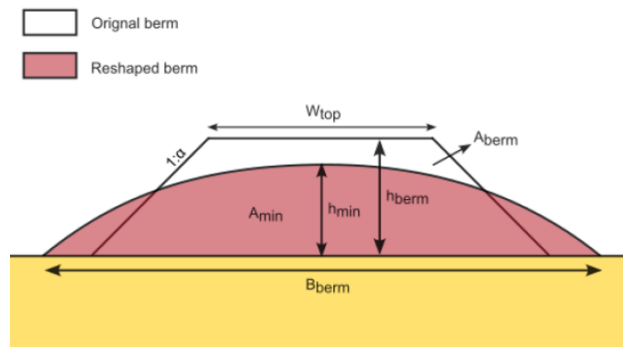
Figure 5.6: Installed trapezoidal berm and reshaped parabolic profile, defining W_{TOP} , the side slope 1:\alpha , h_{berm} , h_{min} , B_{berm} , A_{berm} and A_{min} (Deltaport, 2023).
