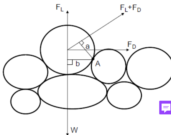
Figure 4.2: Moment equilibrium of a grain around its pivot point A, the drag and lift torque against the torque of the submerged weight. Adapted from Romano (lecture notes).
