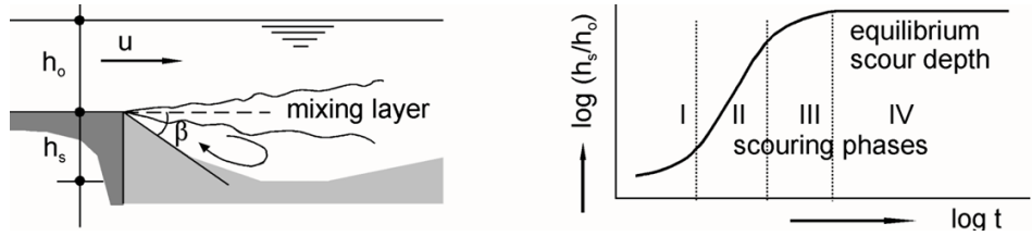
Figure 6.1: The mixing layer above a bed protection and the four scour phases I to IV against time. After Schierck and Verhagen (2019). h_o, u, h_s, \beta, h_s/h_o
