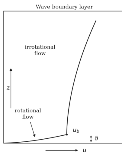
Figure 3.4: Velocity profile under a wave crest, with the thin rotational layer of thickness \delta that carries the wave shear stress (Schiereck and Verhagen, 2019, Fig. 7-7).
