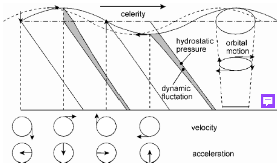
Figure 3.2: Water motion in a periodic non-breaking wave, with the celerity, the pressure and the orbital motion (Schierack and Verhagen, 2019, Fig. 7-3).
