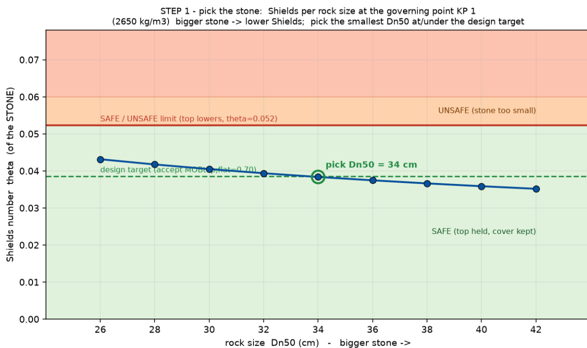
Figure 7.5: Step 1, the Shields number against the stone size at the governing point, from which the smallest safe stone is read.
