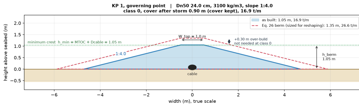
Figure 8.10: Cross-section of the high-density design of Project C at KP 1, before and after the storm, at the height Equation 5.36 asks for at the proposed side slope of 1:4.
