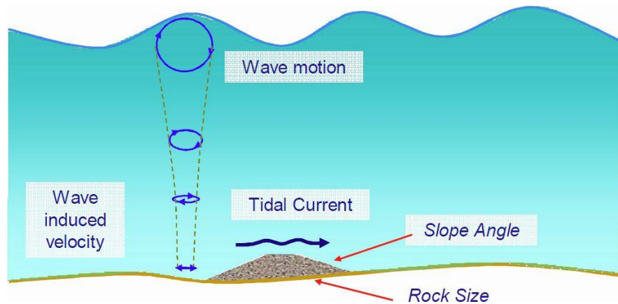
Figure 3.1: Rock berm stability analysis at a cable crossing (specialist design report, 2024).
