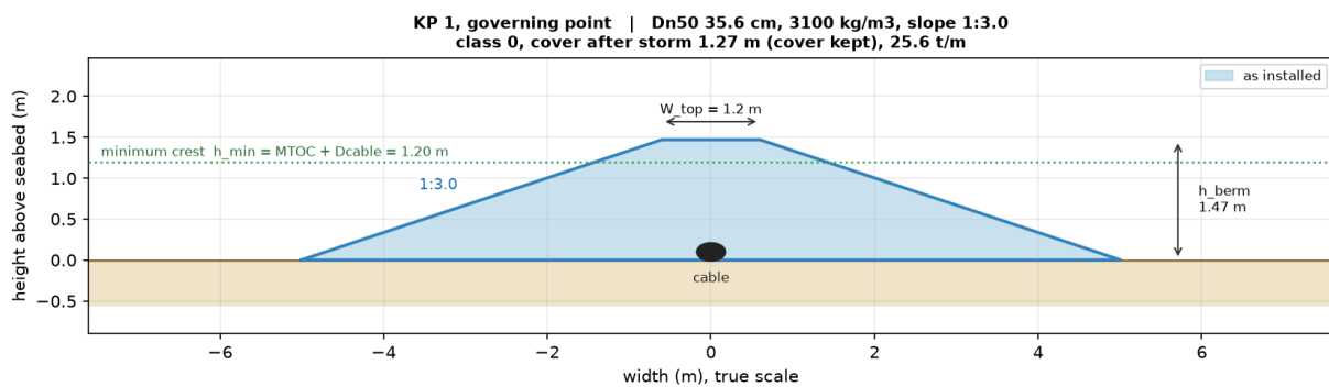
Figure 8.3: Cross-section of the berm as installed for Project A at KP 1. The berm is class 0, so the as-built and the post-storm profile are the same.
