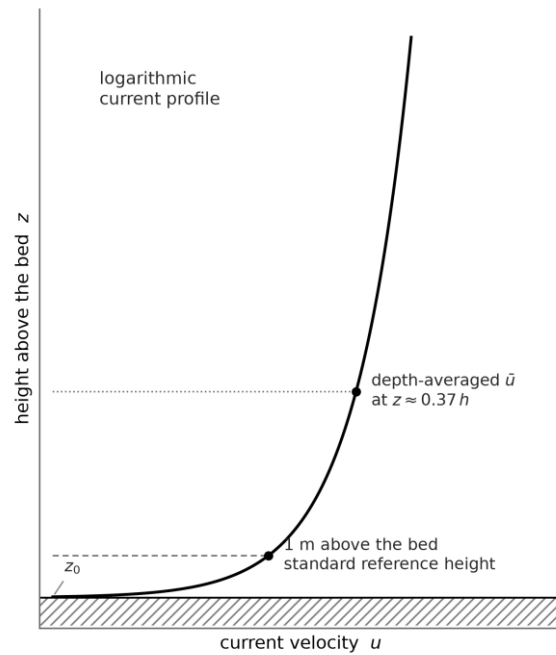
Figure 3.6: Logarithmic velocity profile of a steady current, with the one-metre reference height and the depth-averaged level at about 0.37 h. Own figure, after Schiereck and Verhagen (2019).
