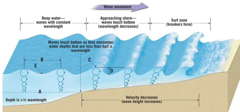
Figure 2.1: The zones of the nearshore environment, from the offshore zone through the shoaling zone to the surf zone (Romano, Lecture Notes Coastal and Harbour Engineering, 2026).
