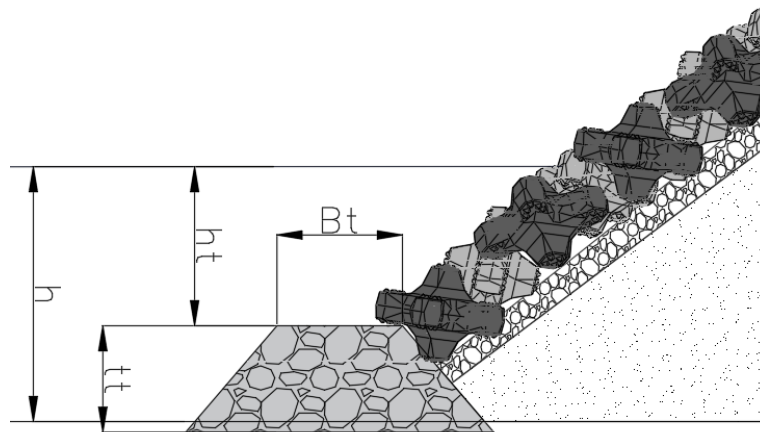
Figure 5.4: Toe berm geometry defining the water depth h , the depth above the toe h_t , the berm width B_t and the berm thickness t_t . (W.Pol drawing).
