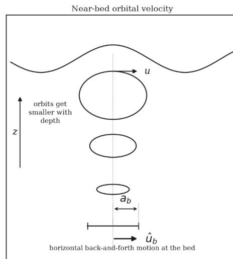
Figure 3.3: Near-bed orbital motion under a wave, with the excursion amplitude a_b and the peak near-bed orbital velocity \hat{u}_b . Own figure, after Schiereck and Verhagen (2019).
